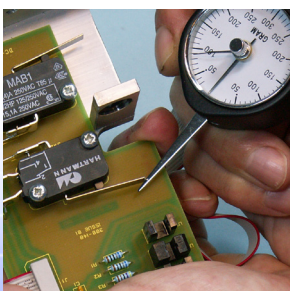
Microswitch Test
